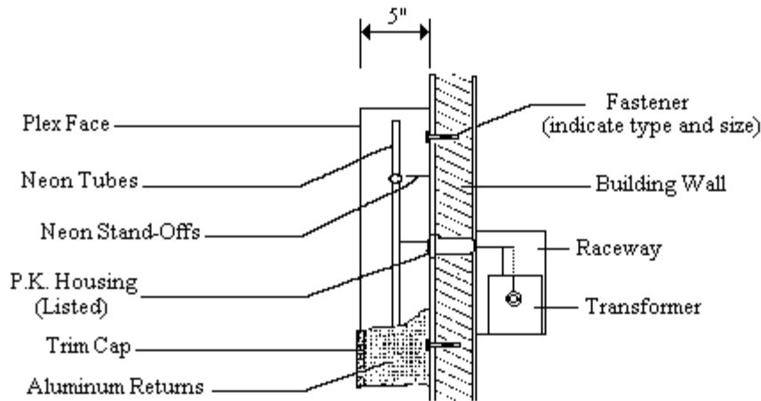
Letters Mounting Detail (U.L. Listed)
